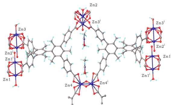
Fig.4 Compusul TCMES-Zn 7 ( 1 )
