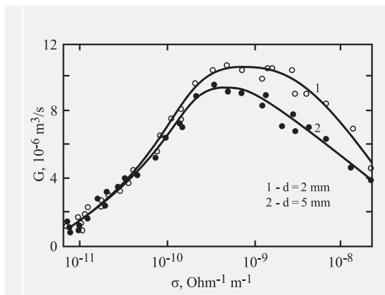
Fig. 7. The dependence of flow rate on conductivity of medium at different distances between electrodes
