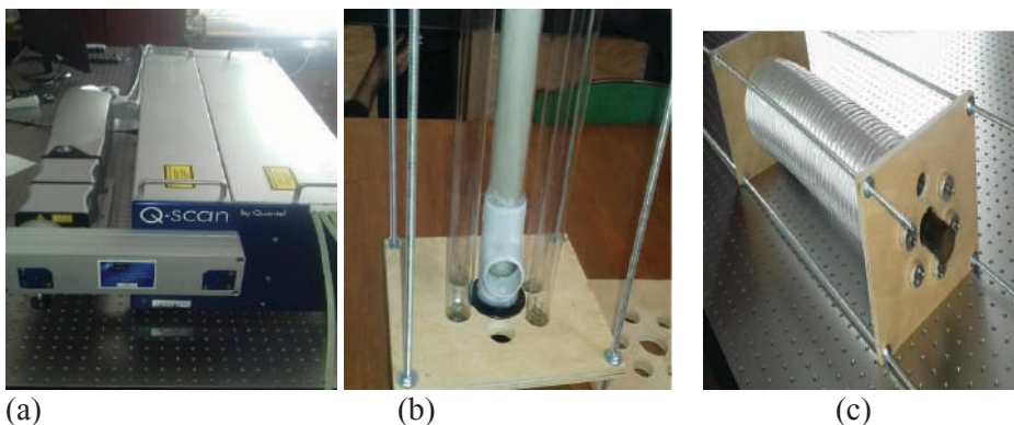
Figure 7. The preparation of mixed decontamination equipment, which use the UVC lamps and laser pulses (a). On the bottom part of the figure is applied the canal for laser beam represented by black circle (b). The final version of decontamination equipment in which laser pulses are sent through the black part of central core (c).
