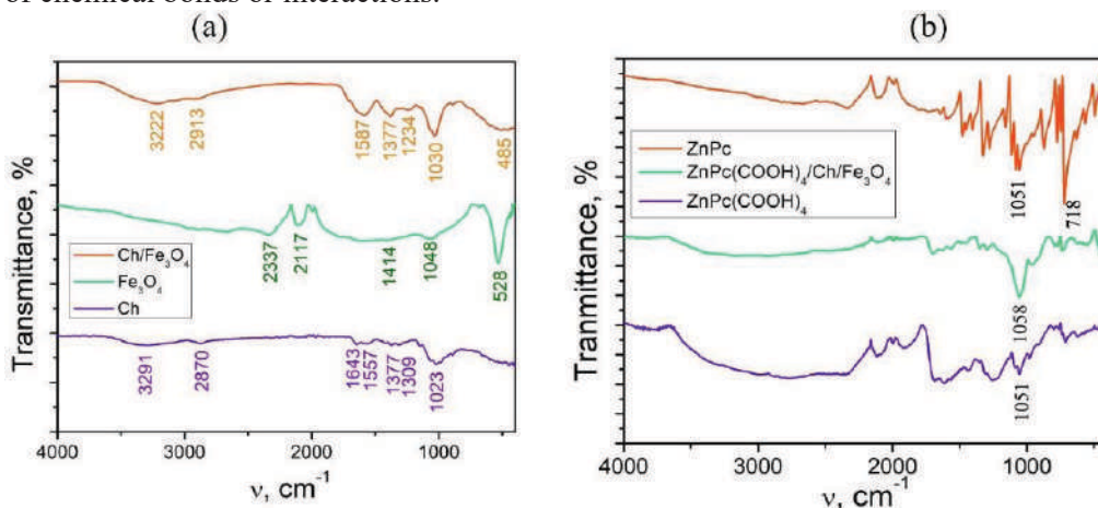
Figure 1. The FTIR spectra of Ch, Fe 3 O 4 , Ch/Fe 3 O 4 NPs (a) and ZnPc, ZnPc(COOH) 4 , ZnPc(COOH) 4 /Ch/Fe 3 O 4 (b)
