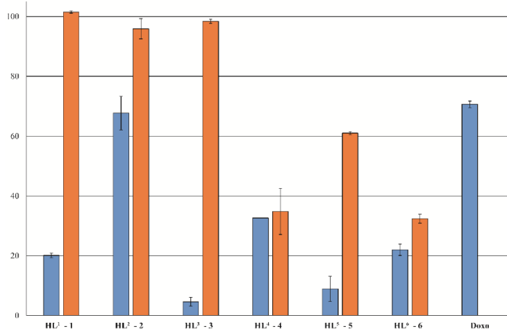
Figure 4. Antiproliferative activity of the synthesized thiosemicarbazones and their copper(II) complexes against the human prostate cancer PC-3 cell line at 10 \mu M
