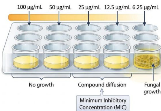
Figure 4. Determination of the minimum inhibitory concentration (MIC) by the microdilution method: variation of compound concentration in wells and assessment of fungal growth inhibition
