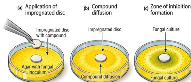
Figure 3. Schematic representation of the disc diffusion method for the evaluation of antifungal activity: (a) application of the compound-impregnated disc onto the inoculated medium, (b) diffusion of the compound into the agar, (c) formation of the inhibition zone.
