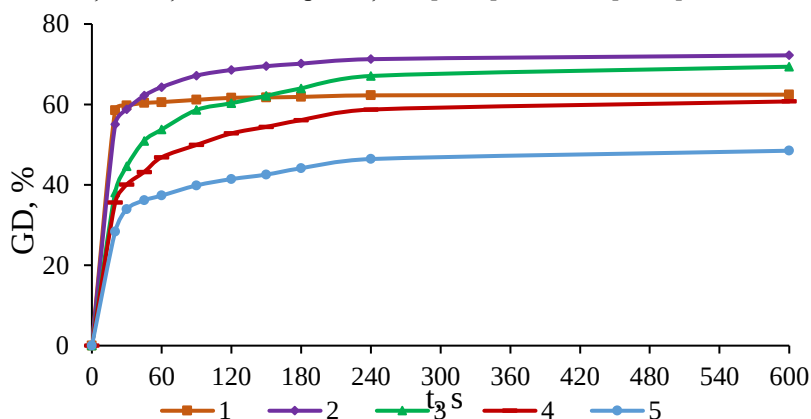
Figura 6. Dependenta \text{GD} = f(t) în cazul sistemului Fenton: 1 - \frac{[\text{H}_2\text{O}_2]}{[\text{Fe}^{2+}]} = 5 ; 2 - \frac{[\text{H}_2\text{O}_2]}{[\text{Fe}^{2+}]} = 10 ; 3 - \frac{[\text{H}_2\text{O}_2]}{[\text{Fe}^{2+}]} = 20 ; 4 - \frac{[\text{H}_2\text{O}_2]}{[\text{Fe}^{2+}]} = 30 ; 5 - \frac{[\text{H}_2\text{O}_2]}{[\text{Fe}^{2+}]} = 50
