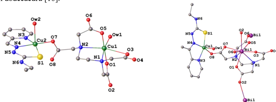
Figura 5. Structura complexului a) homometalic [Cu(HFoPyTSC-4Et)Cu(edta)] \cdot 3.5H_2O b) heterometalic \{[Cu(AcPyTSC-Et)Bi(edta)] \cdot 5H_2O\}_n [10]
