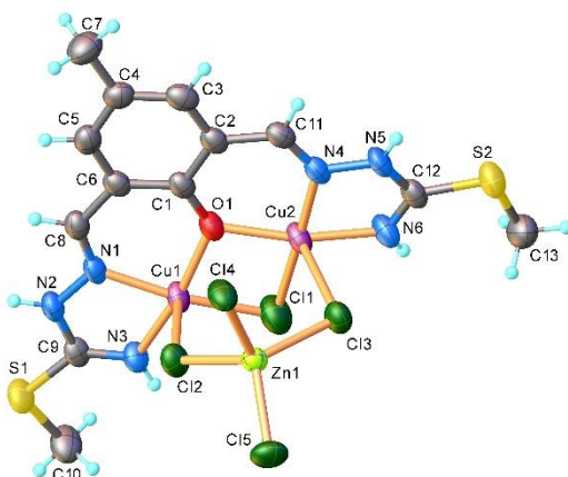
Figure 2. X-ray molecular structure of [\text{Cu}_2\text{H}_2\text{Q}-\mu\text{-Cl}-\mu\text{-(ZnCl}_4\text{)}] ( 4 ) with atom labelling and thermal ellipsoids at 50% level.
