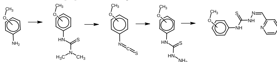
Figure 1. Synthetic scheme of thiosemicarbazones HL 1 –HL 3
