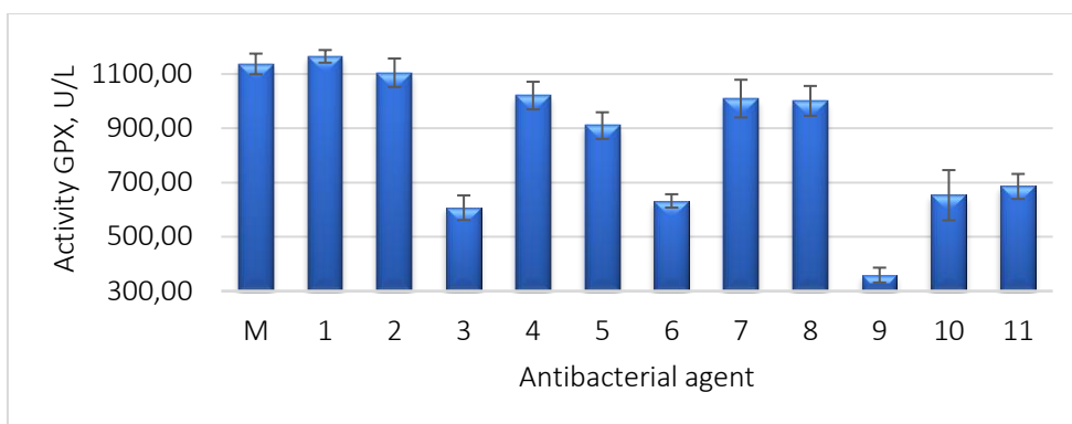
Figure 5. Influence of tested compounds on glutathione peroxidase activity in S. aureus
