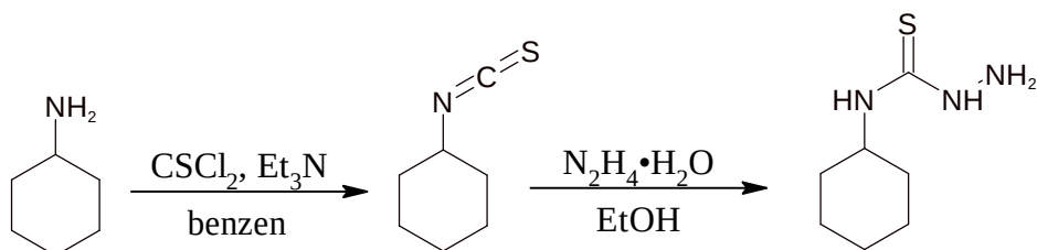
Figure 3. Synthesis scheme of N -cyclohexylhydrazinecarbothioamide from amine
