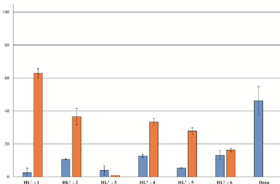
Figure 5. Antiproliferative activity of the synthesized thiosemicarbazones and their copper(II) complexes against the human colorectal cancer HT-29 cell line at 10 μM
