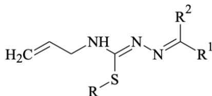
Figure 1. The structural formula of isothiosemicarbazones.
