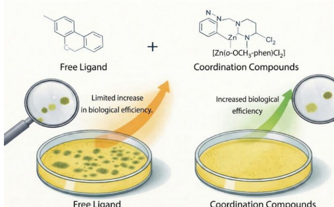
Figure 6. Comparative representation of antifungal activity: free ligand versus coordination complexes, highlighting the increase in biological efficacy
