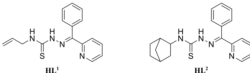
Figure 1. The structural formula of 2-benzoylpyridine 4-allyl/norbornylthiosemicarbazones (HL 1-2 )
