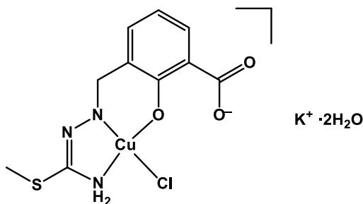
Figure 10. Water-soluble monopotassium salt of complex 6 .
