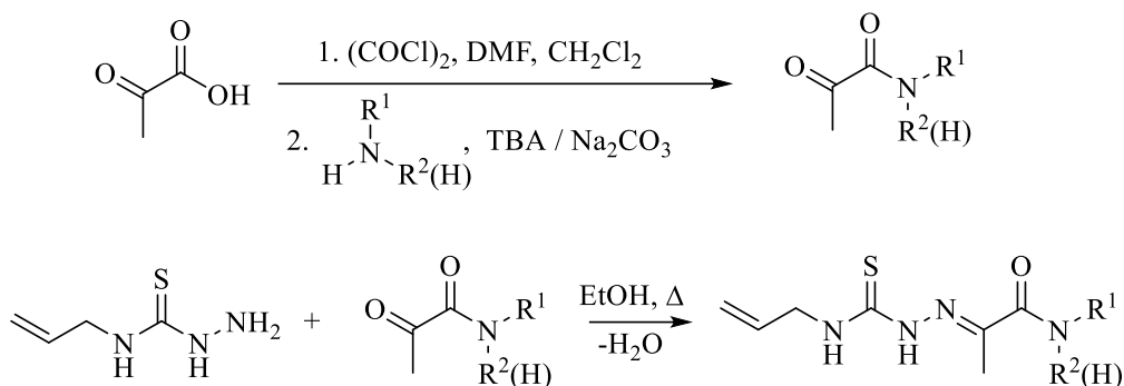
Figure 2. Synthesis of pyruvamide 4-allylthiosemicarbazones HL 1-6
